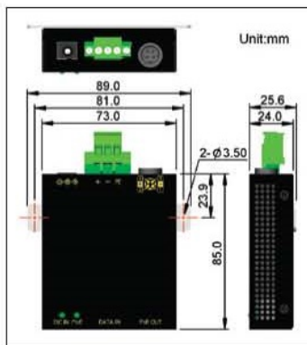
Panel Dimension
