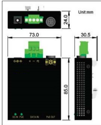
DIN-Rail Dimension
